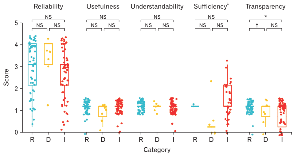
Supplement 3. Comparison of the quality scores between the categories and domains (N=116). P-values were calculated by Wilcoxon-Mann-Whitney test. NS, not studied due to tied values (not significant); R, risk factor; D, diagnosis; I, Intervention. *P=0.00081. †P=0.012. ‡N=38.
